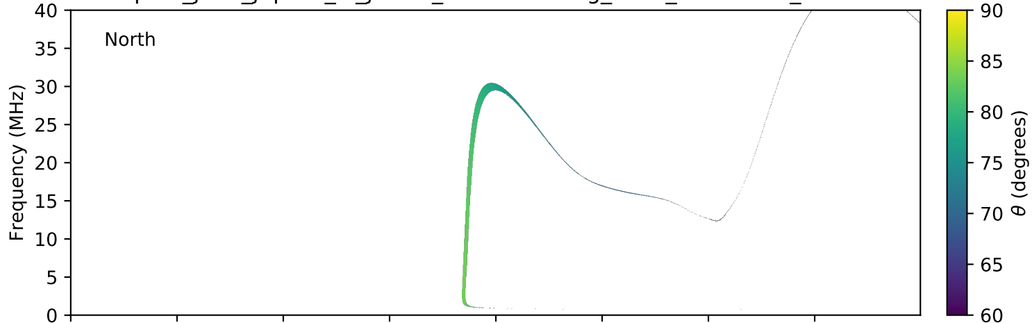
expres_juno_jupiter_io_jrm09_lossc-wid1deg_3kev_20170701_v01.cdf
