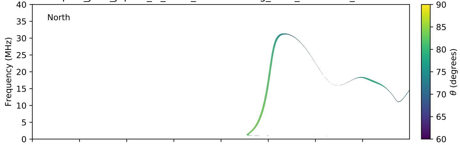
expres_juno_jupiter_io_isaac_lossc-wid1deg_3kev_20170731_v01.cdf
