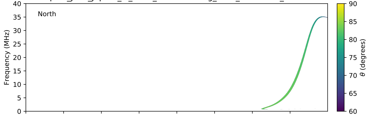
expres_juno_jupiter_io_isaac_lossc-wid1deg_3kev_20170729_v01.cdf
