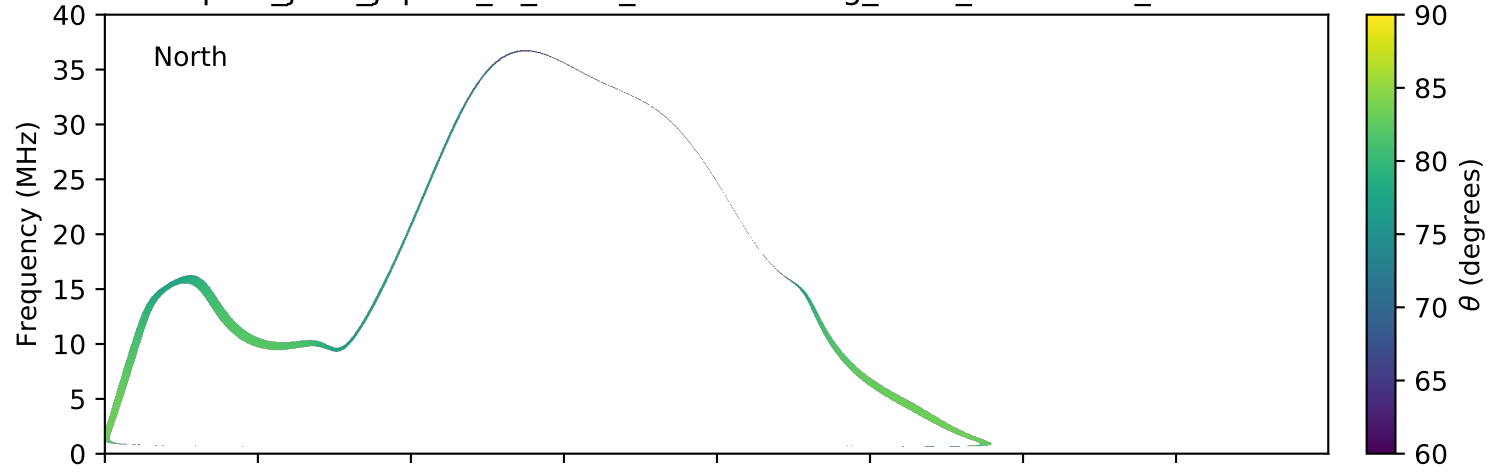
expres_juno_jupiter_io_isaac_lossc-wid1deg_3kev_20170728_v01.cdf
