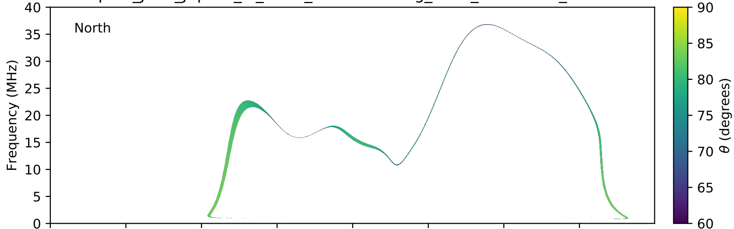
expres_juno_jupiter_io_isaac_lossc-wid1deg_3kev_20170726_v01.cdf
