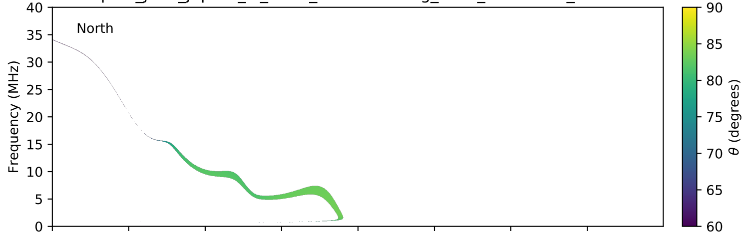
expres_juno_jupiter_io_isaac_lossc-wid1deg_3kev_20170723_v01.cdf
