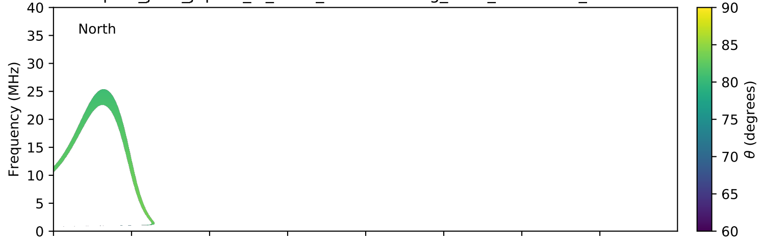
expres_juno_jupiter_io_isaac_lossc-wid1deg_3kev_20170718_v01.cdf
