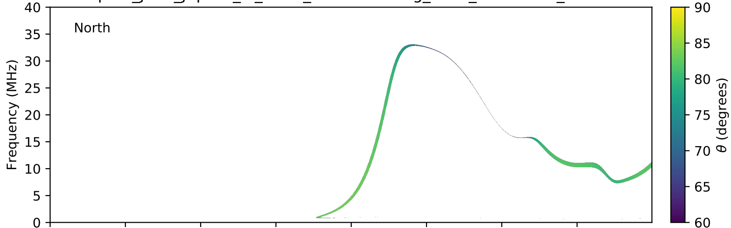
expres_juno_jupiter_io_isaac_lossc-wid1deg_3kev_20170717_v01.cdf
