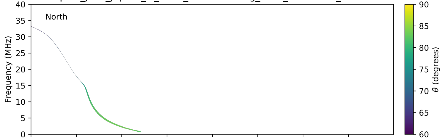
expres_juno_jupiter_io_isaac_lossc-wid1deg_3kev_20170716_v01.cdf
