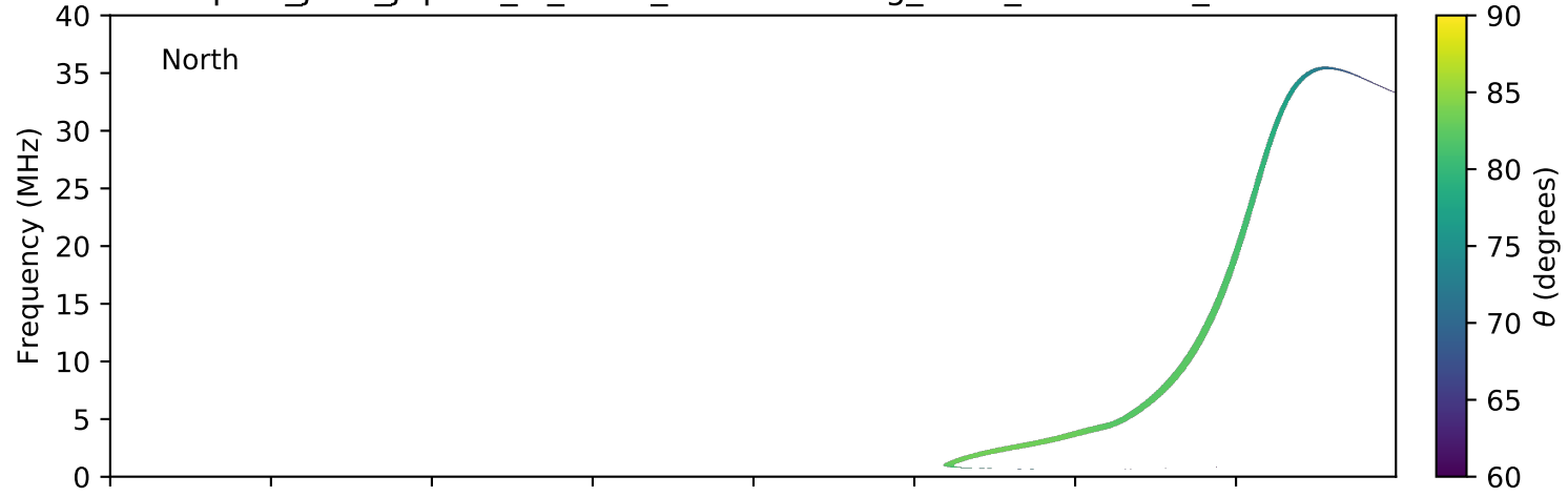
expres_juno_jupiter_io_isaac_lossc-wid1deg_3kev_20170715_v01.cdf
