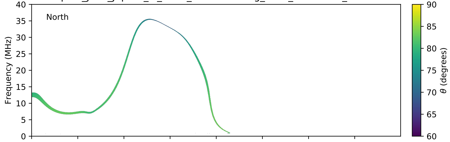
expres_juno_jupiter_io_isaac_lossc-wid1deg_3kev_20170714_v01.cdf
