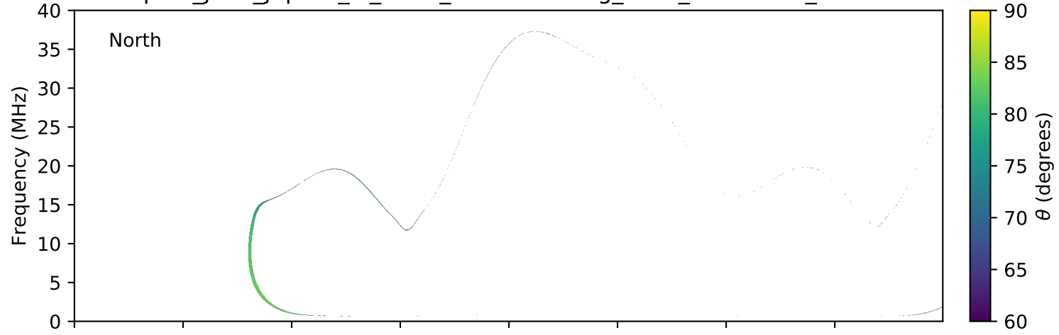
expres_juno_jupiter_io_isaac_lossc-wid1deg_3kev_20170710_v01.cdf
