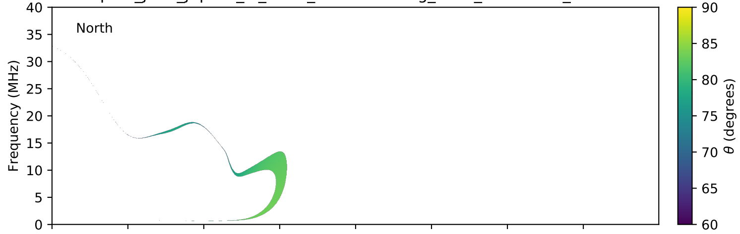
expres_juno_jupiter_io_isaac_lossc-wid1deg_3kev_20170709_v01.cdf
