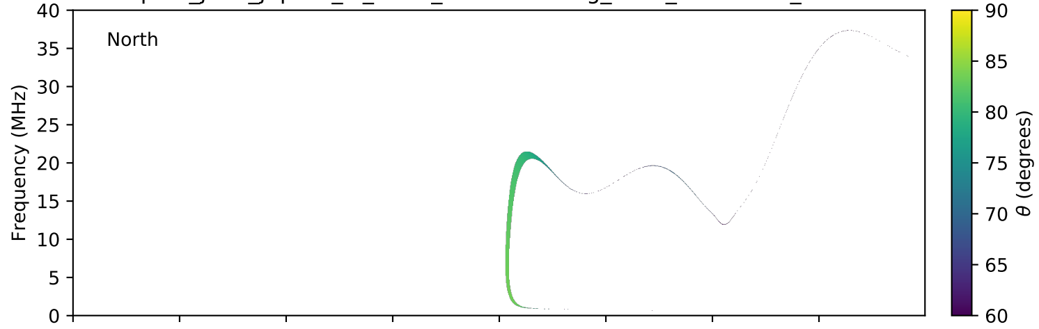
expres_juno_jupiter_io_isaac_lossc-wid1deg_3kev_20170708_v01.cdf
