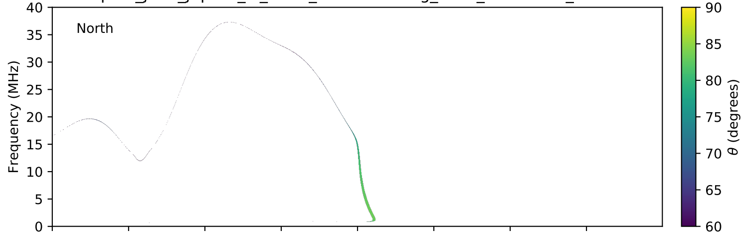
expres_juno_jupiter_io_isaac_lossc-wid1deg_3kev_20170707_v01.cdf
