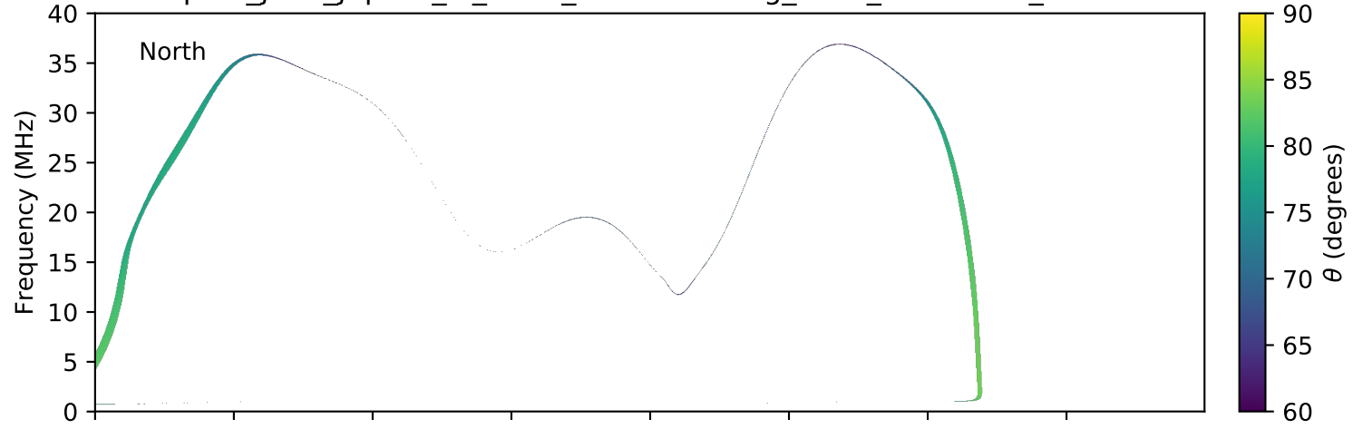
expres_juno_jupiter_io_isaac_lossc-wid1deg_3kev_20170705_v01.cdf
