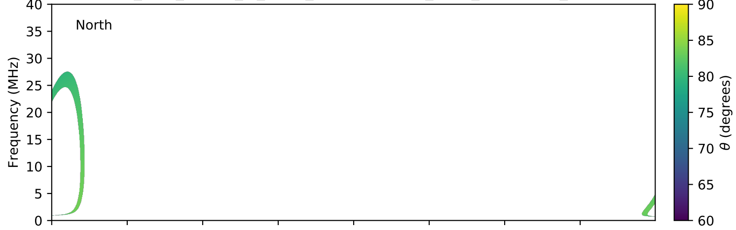
expres_juno_jupiter_io_isaac_lossc-wid1deg_3kev_20170704_v01.cdf
