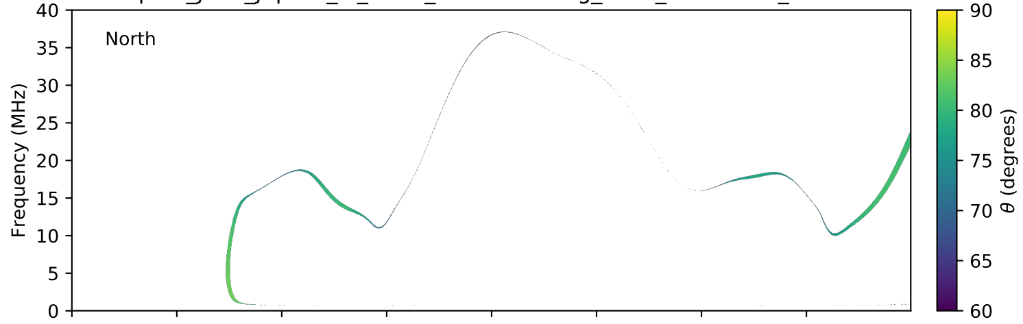
expres_juno_jupiter_io_isaac_lossc-wid1deg_3kev_20170703_v01.cdf
