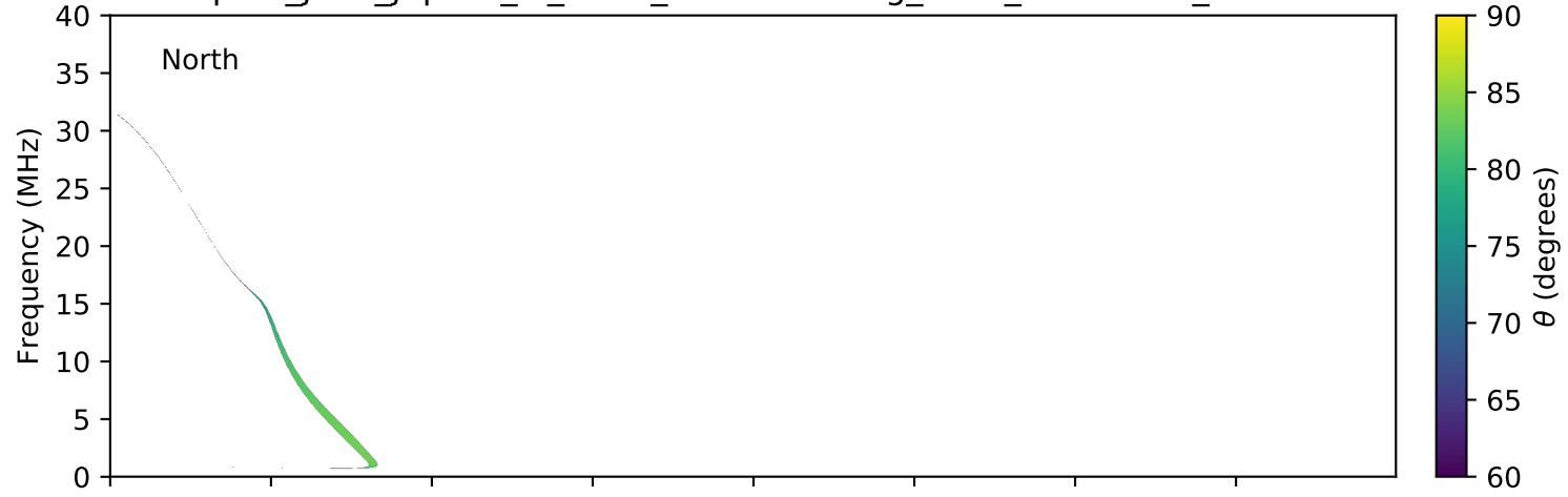
expres_juno_jupiter_io_isaac_lossc-wid1deg_3kev_20170702_v01.cdf
