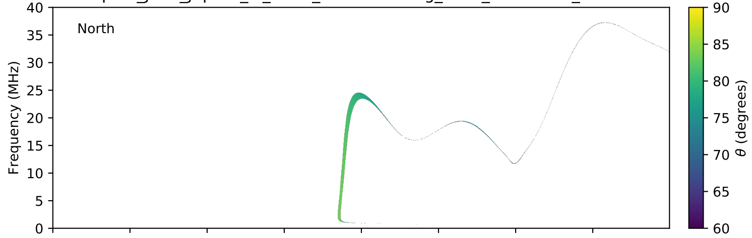
expres_juno_jupiter_io_isaac_lossc-wid1deg_3kev_20170701_v01.cdf
