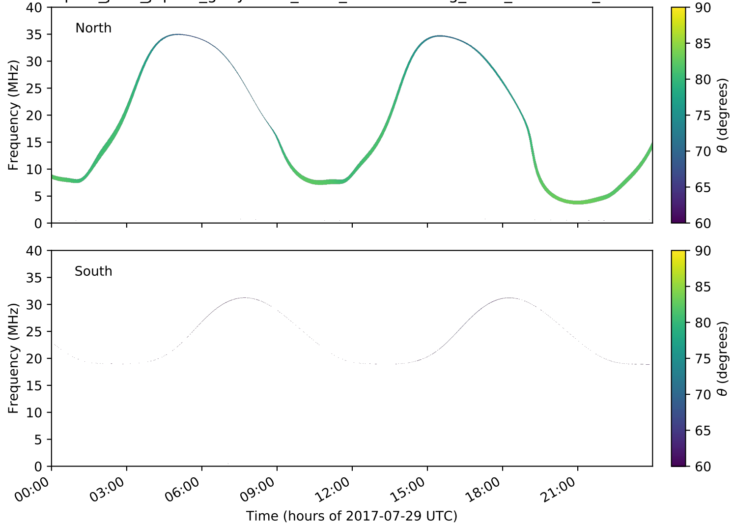
expres_juno_jupiter_ganymede_isaac_lossc-wid1deg_3kev_20170729_v01.cdf
