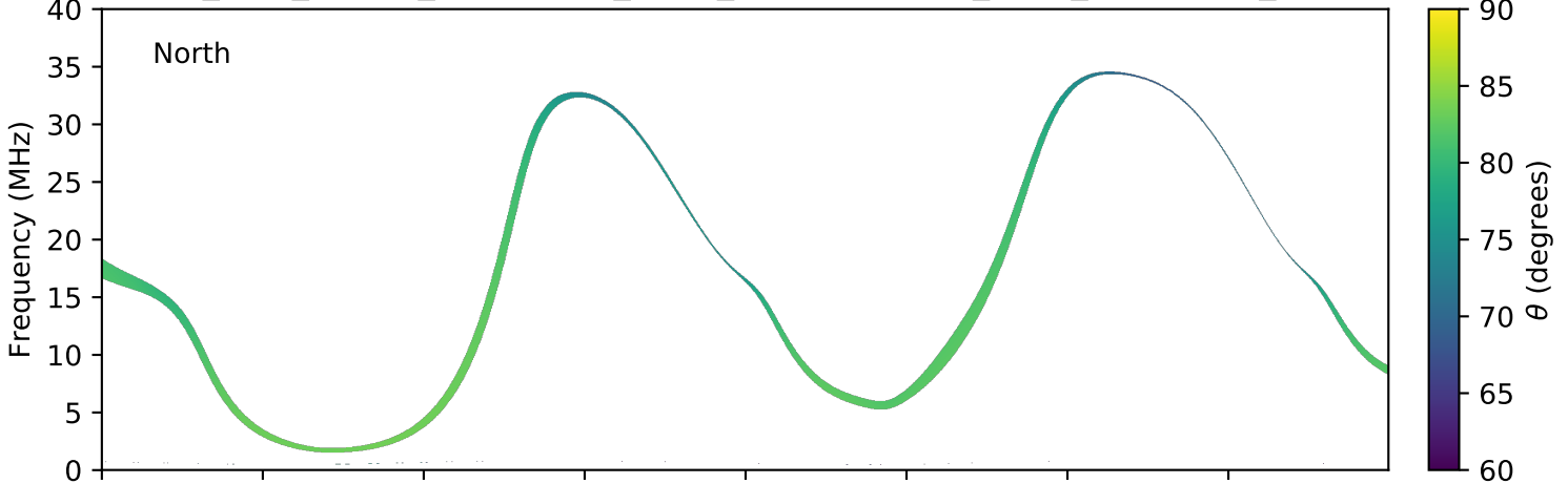
expres_juno_jupiter_ganymede_isaac_lossc-wid1deg_3kev_20170728_v01.cdf
