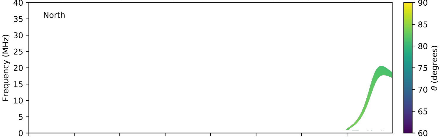
expres_juno_jupiter_ganymede_isaac_lossc-wid1deg_3kev_20170727_v01.cdf
