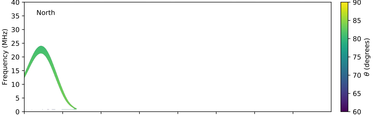
expres_juno_jupiter_ganymede_isaac_lossc-wid1deg_3kev_20170723_v01.cdf
