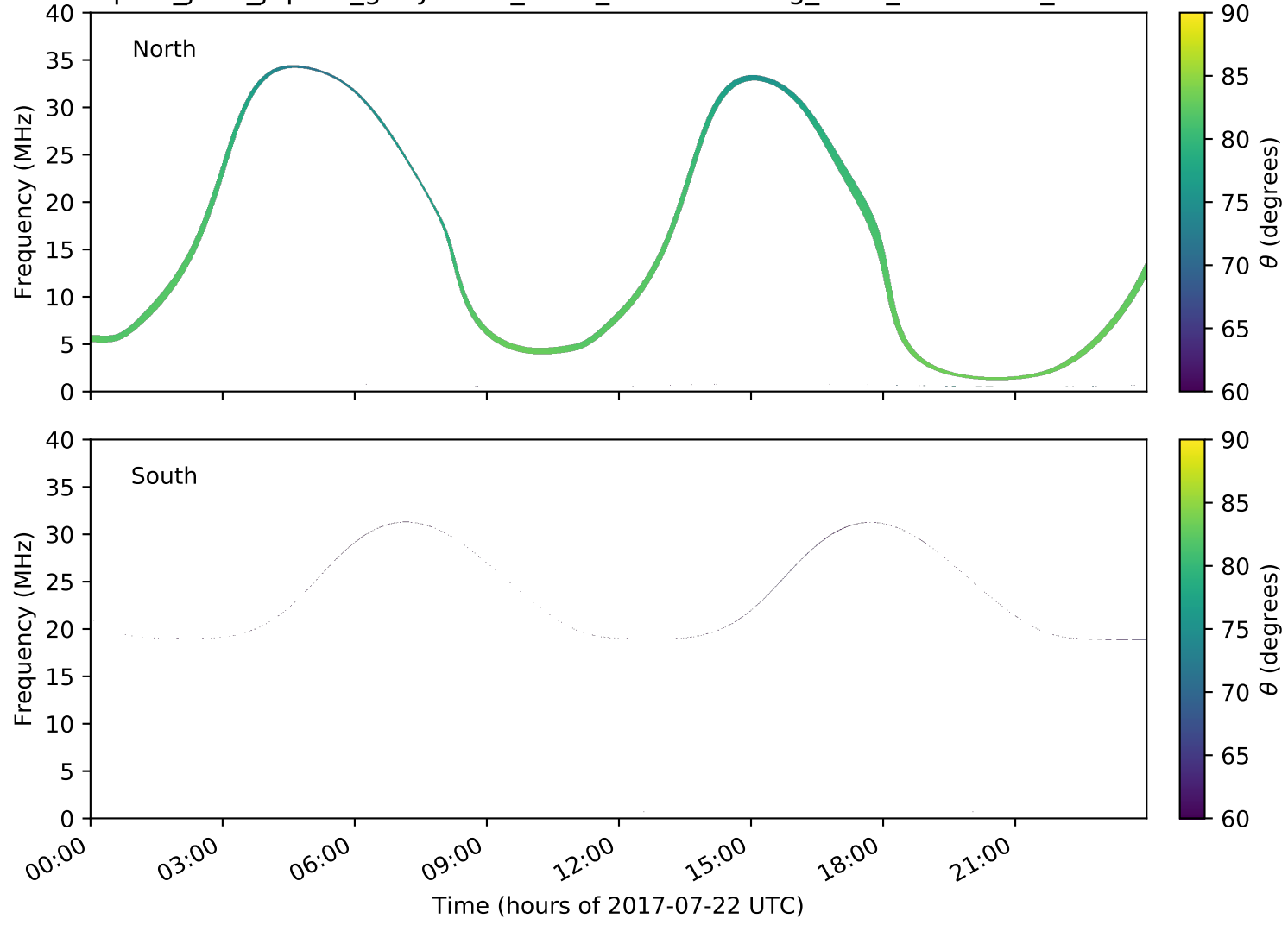
expres_juno_jupiter_ganymede_isaac_lossc-wid1deg_3kev_20170722_v01.cdf
