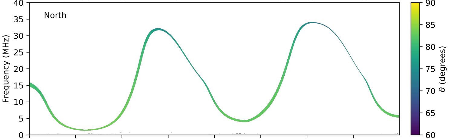
expres_juno_jupiter_ganymede_isaac_lossc-wid1deg_3kev_20170721_v01.cdf
