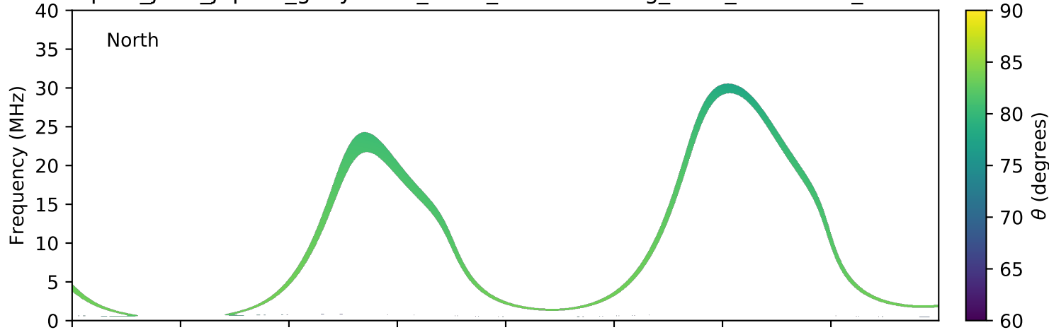
expres_juno_jupiter_ganymede_isaac_lossc-wid1deg_3kev_20170714_v01.cdf
