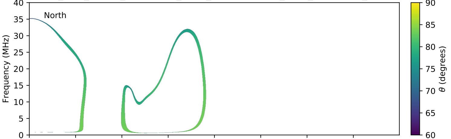
expres_juno_jupiter_ganymede_isaac_lossc-wid1deg_3kev_20170709_v01.cdf
