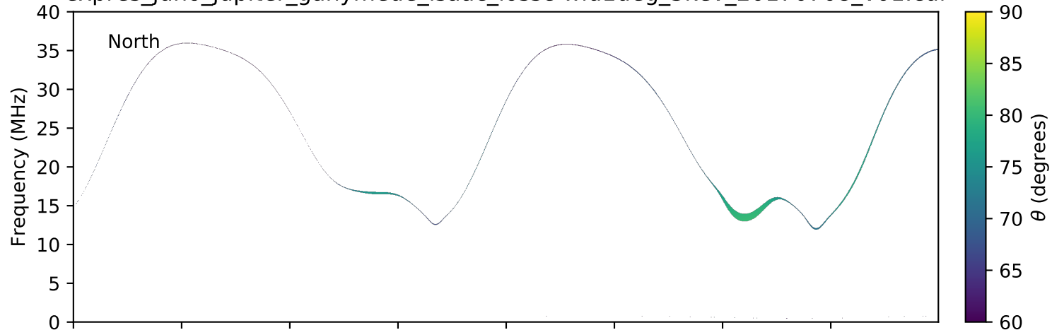
expres_juno_jupiter_ganymede_isaac_lossc-wid1deg_3kev_20170708_v01.cdf
