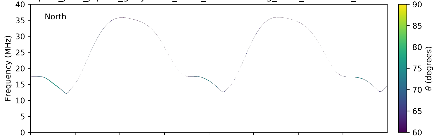
expres_juno_jupiter_ganymede_isaac_lossc-wid1deg_3kev_20170707_v01.cdf
