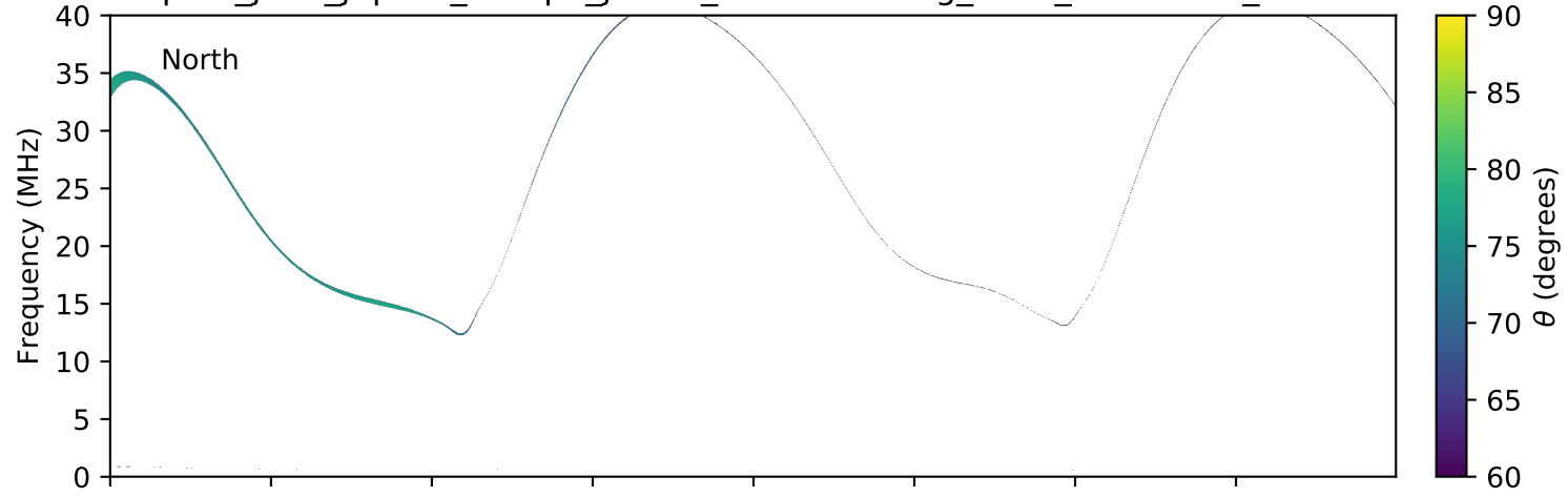
expres_juno_jupiter_europa_jrm09_lossc-wid1deg_3kev_20170706_v01.cdf
