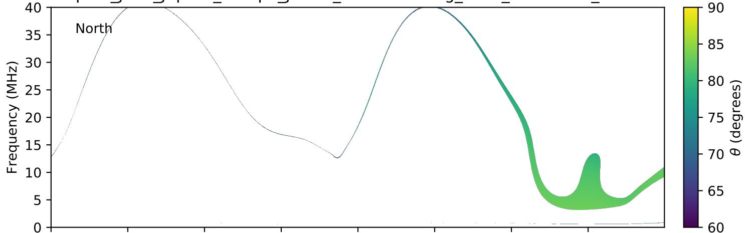
expres_juno_jupiter_europa_jrm09_lossc-wid1deg_3kev_20170703_v01.cdf
