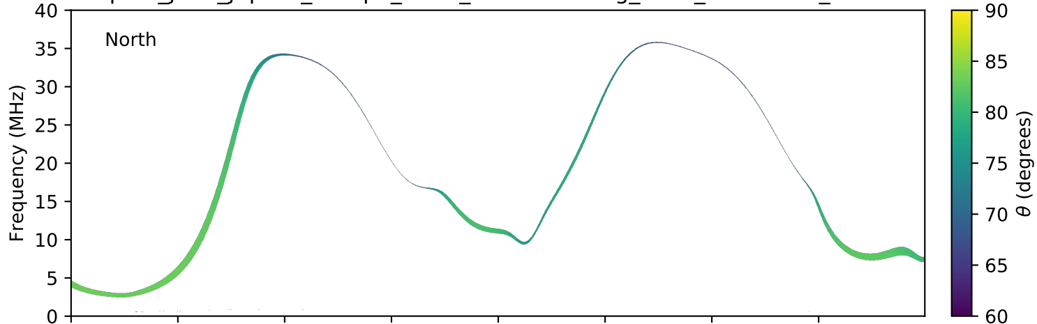
expres_juno_jupiter_europa_isaac_lossc-wid1deg_3kev_20170731_v01.cdf
