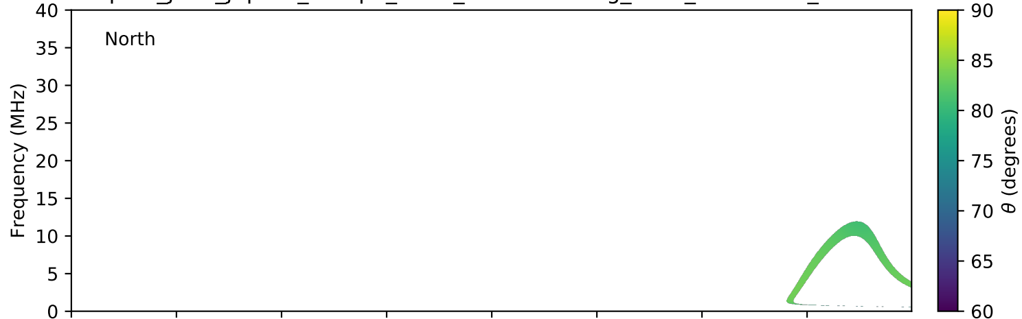
expres_juno_jupiter_europa_isaac_lossc-wid1deg_3kev_20170730_v01.cdf
