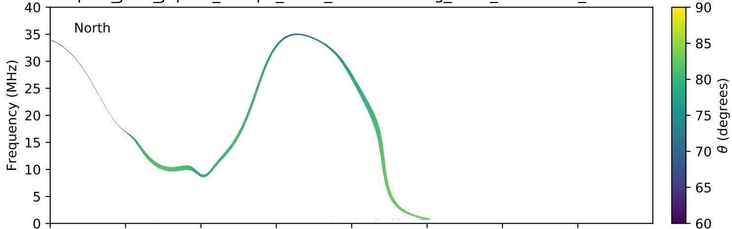
expres_juno_jupiter_europa_isaac_lossc-wid1deg_3kev_20170728_v01.cdf
