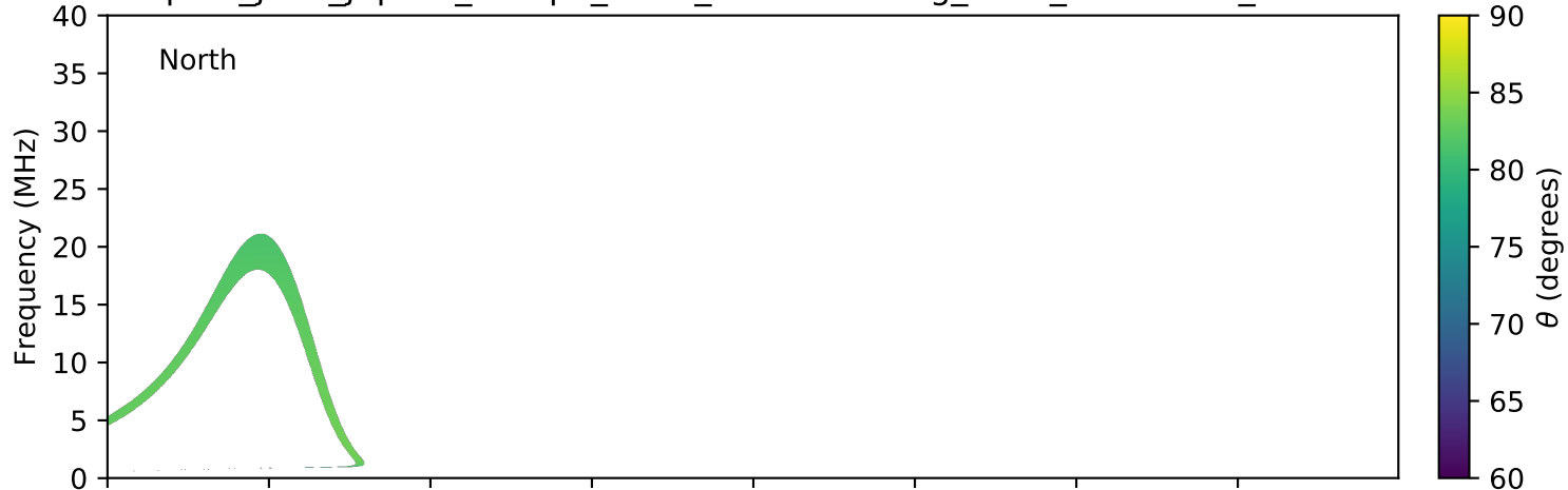
expres_juno_jupiter_europa_isaac_lossc-wid1deg_3kev_20170725_v01.cdf
