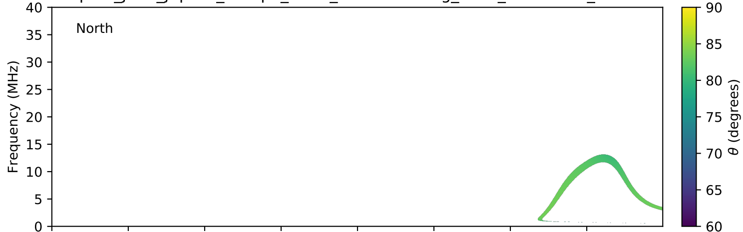
expres_juno_jupiter_europa_isaac_lossc-wid1deg_3kev_20170723_v01.cdf
