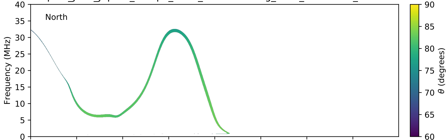
expres_juno_jupiter_europa_isaac_lossc-wid1deg_3kev_20170721_v01.cdf
