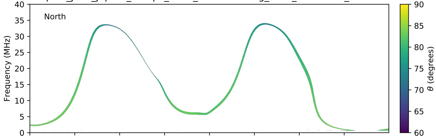
expres_juno_jupiter_europa_isaac_lossc-wid1deg_3kev_20170717_v01.cdf
