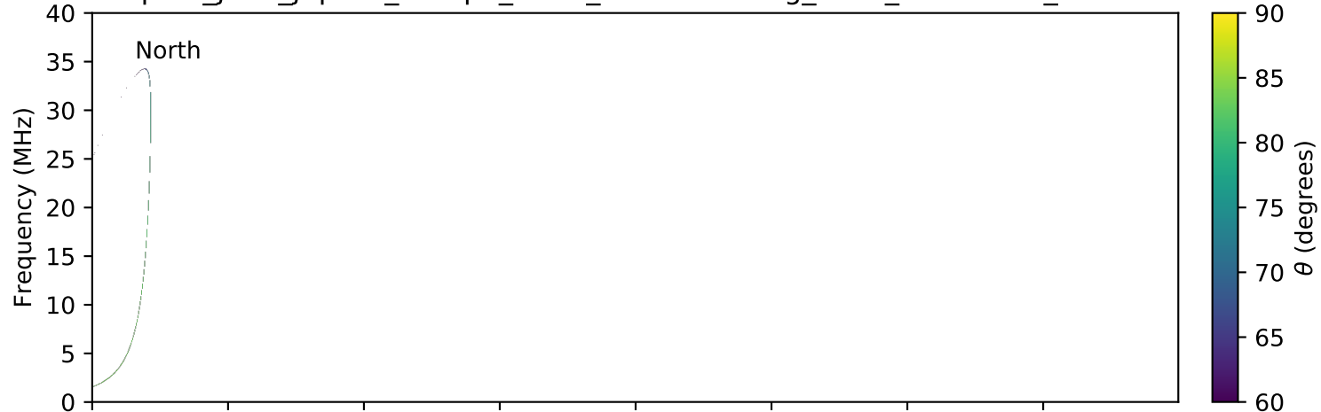
expres_juno_jupiter_europa_isaac_lossc-wid1deg_3kev_20170711_v01.cdf
