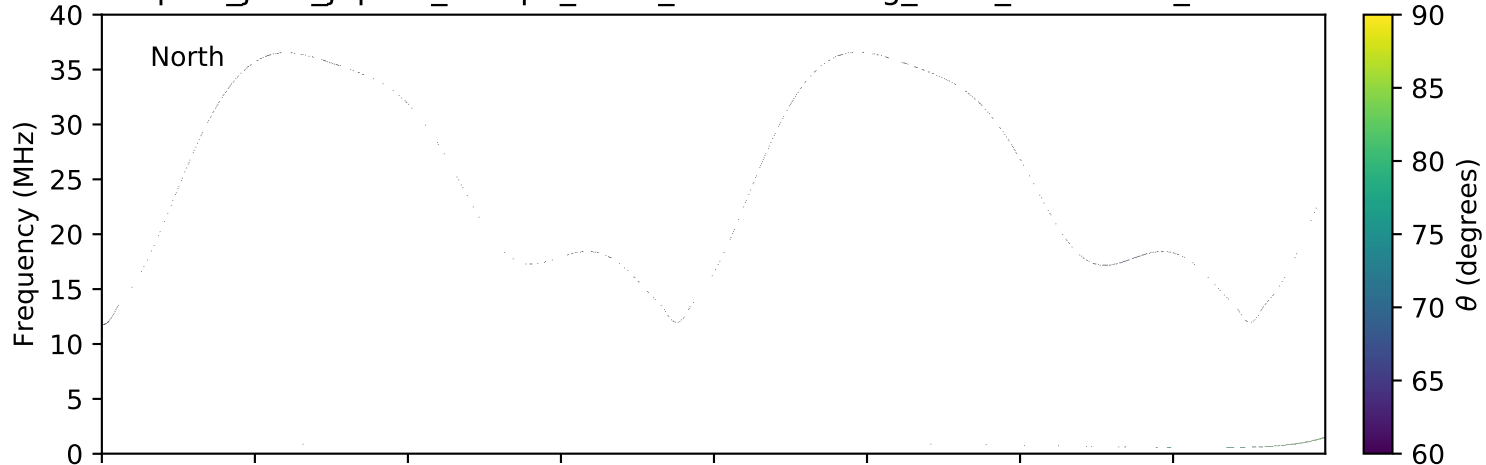
expres_juno_jupiter_europa_isaac_lossc-wid1deg_3kev_20170710_v01.cdf
