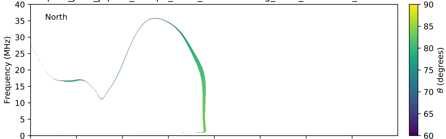
expres_juno_jupiter_europa_isaac_lossc-wid1deg_3kev_20170707_v01.cdf
