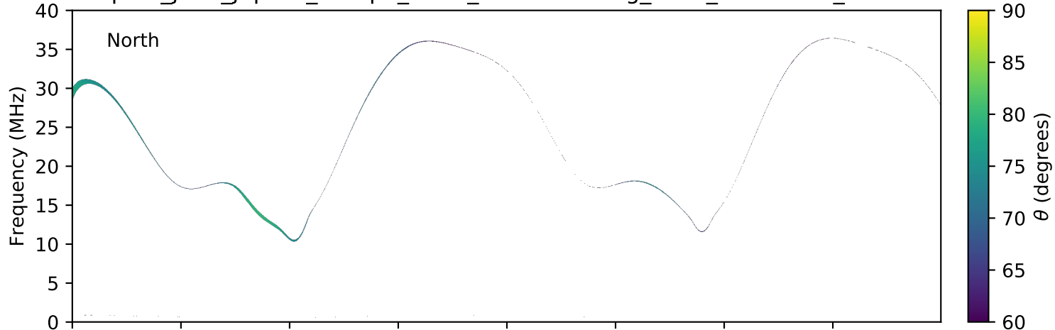
expres_juno_jupiter_europa_isaac_lossc-wid1deg_3kev_20170706_v01.cdf
