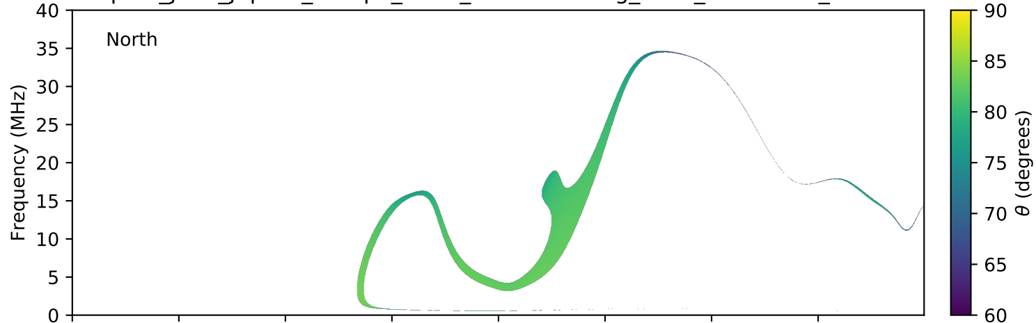
expres_juno_jupiter_europa_isaac_lossc-wid1deg_3kev_20170702_v01.cdf
