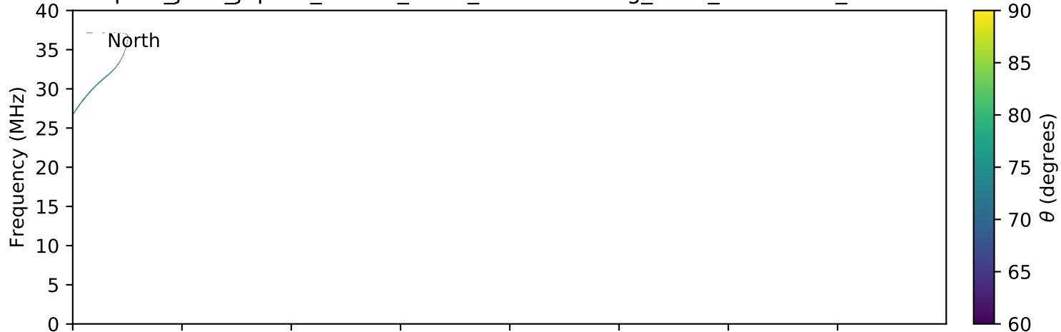
expres_juno_jupiter_75d-0r_isaac_lossc-wid1deg_9kev_20170711_v01.cdf
