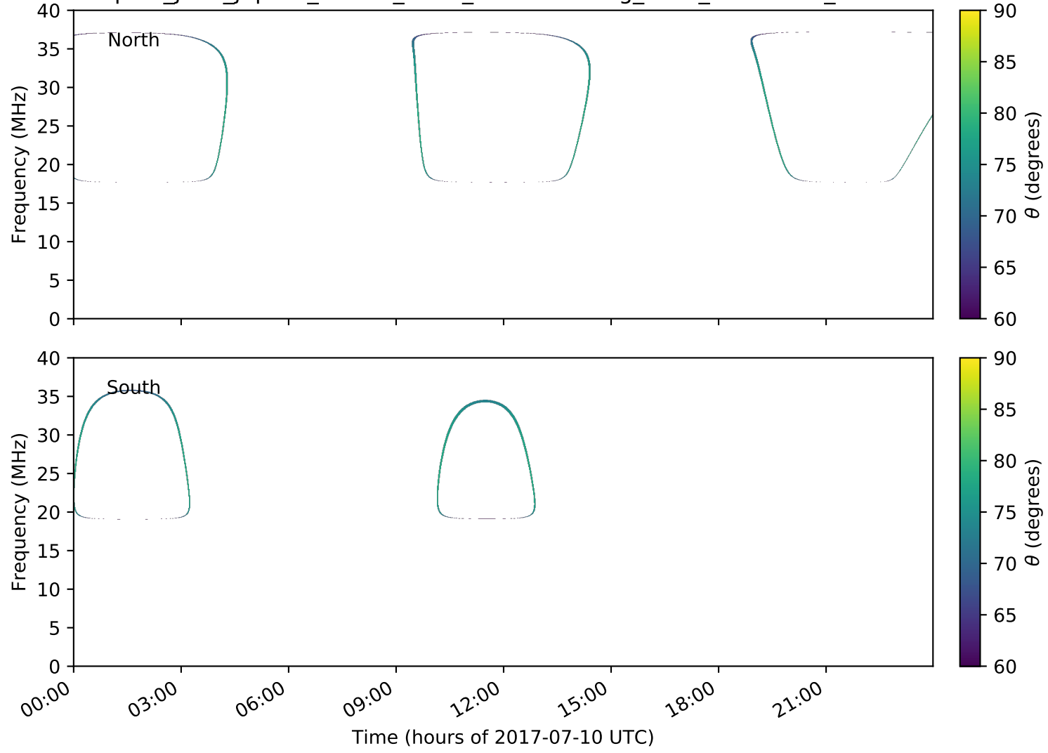
expres_juno_jupiter_75d-0r_isaac_lossc-wid1deg_9kev_20170710_v01.cdf
