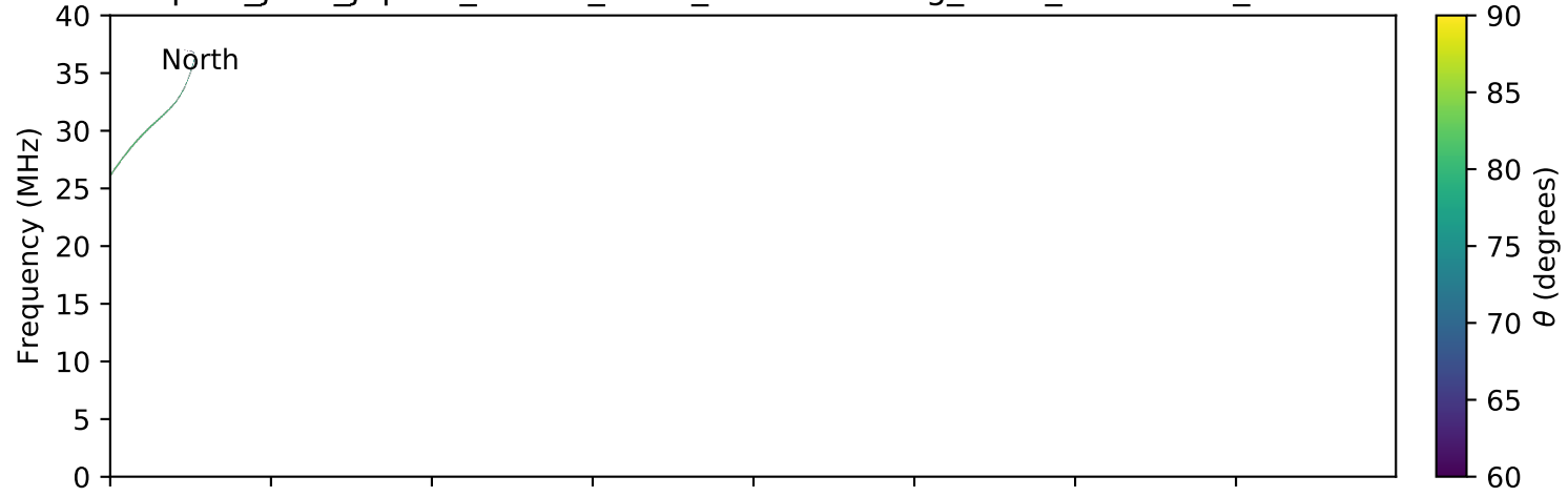
expres_juno_jupiter_75d-0r_isaac_lossc-wid1deg_5kev_20170711_v01.cdf
