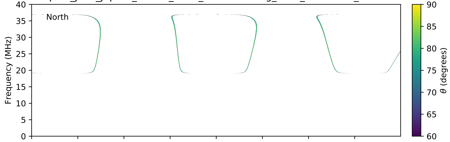
expres_juno_jupiter_75d-0r_isaac_lossc-wid1deg_5kev_20170710_v01.cdf
