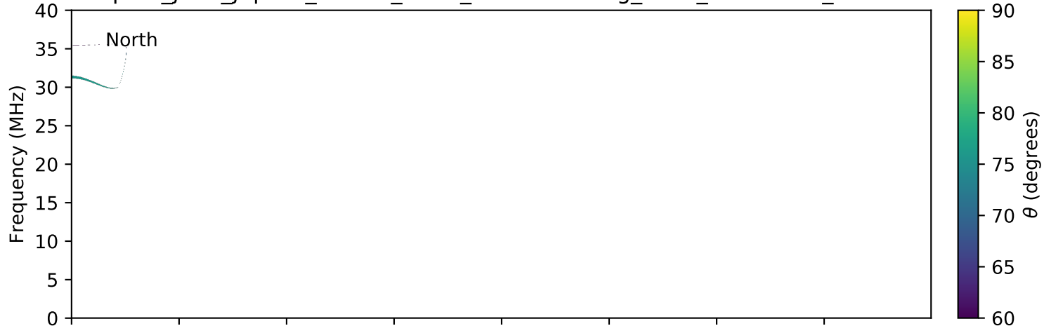
expres_juno_jupiter_17d-0r_isaac_lossc-wid1deg_9kev_20170711_v01.cdf
