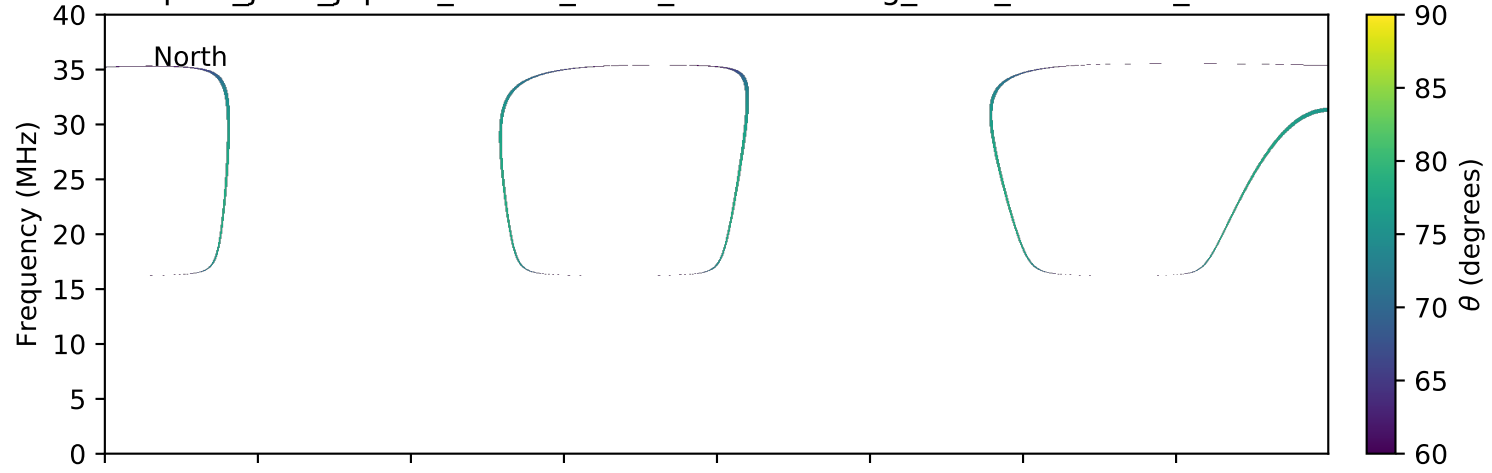
expres_juno_jupiter_17d-0r_isaac_lossc-wid1deg_9kev_20170710_v01.cdf
